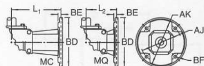
FRAMES 182-184TC, 213-215TC, & 254-256TC
