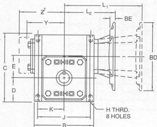
FRAMES 56C & 143-145TC
