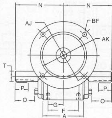
FRAMES 182-184TC, 213-215TC, & 254-256TC
