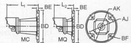
FRAMES 182-184TC, 213-215TC, & 254-256TC
